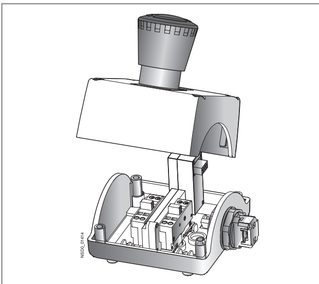
EMERGENCY-STOP enclosure
