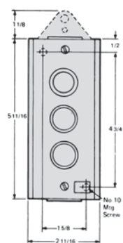
3 Unit Stations Surface Mounting
