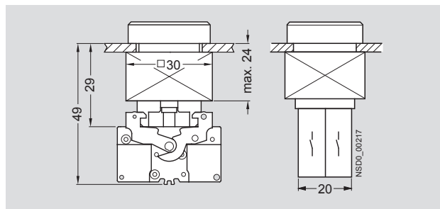
Push button with two contact blocks
